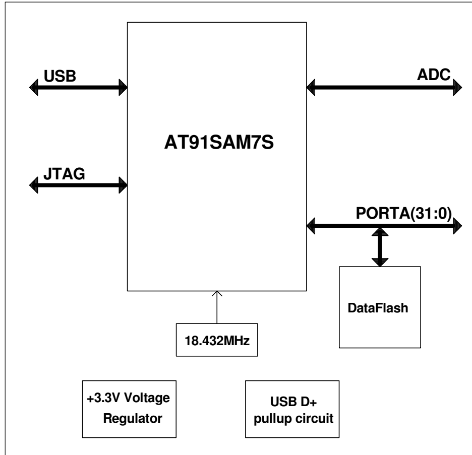
Figure 1 Block diagram of MMsam7s minimodule.
