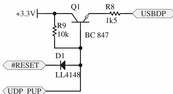
Figure 5 Implementation of D+ pull-up circuit.
