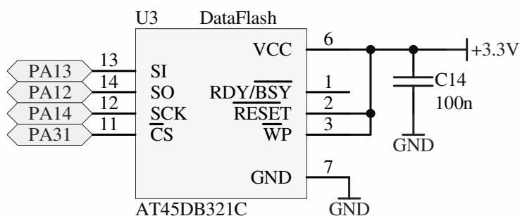
Figure 3 Connection of DataFlash memory inside the module.
