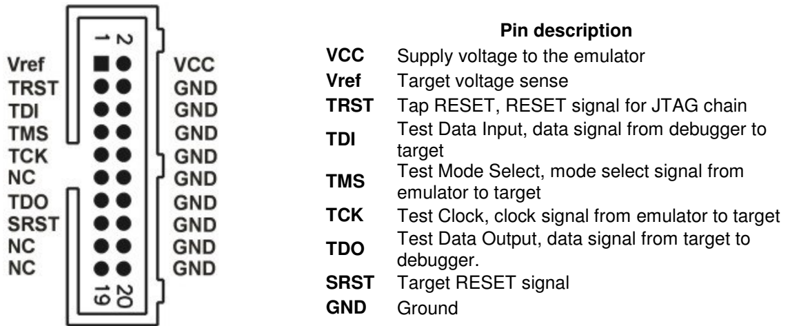
Figure 7 JTAG connector.
