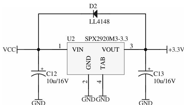
Figure 4 3.3V voltage regulator.
